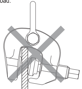
Main body must not be installed in a tilted position.
