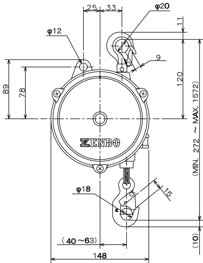
SPRING BALANCER EW-3
