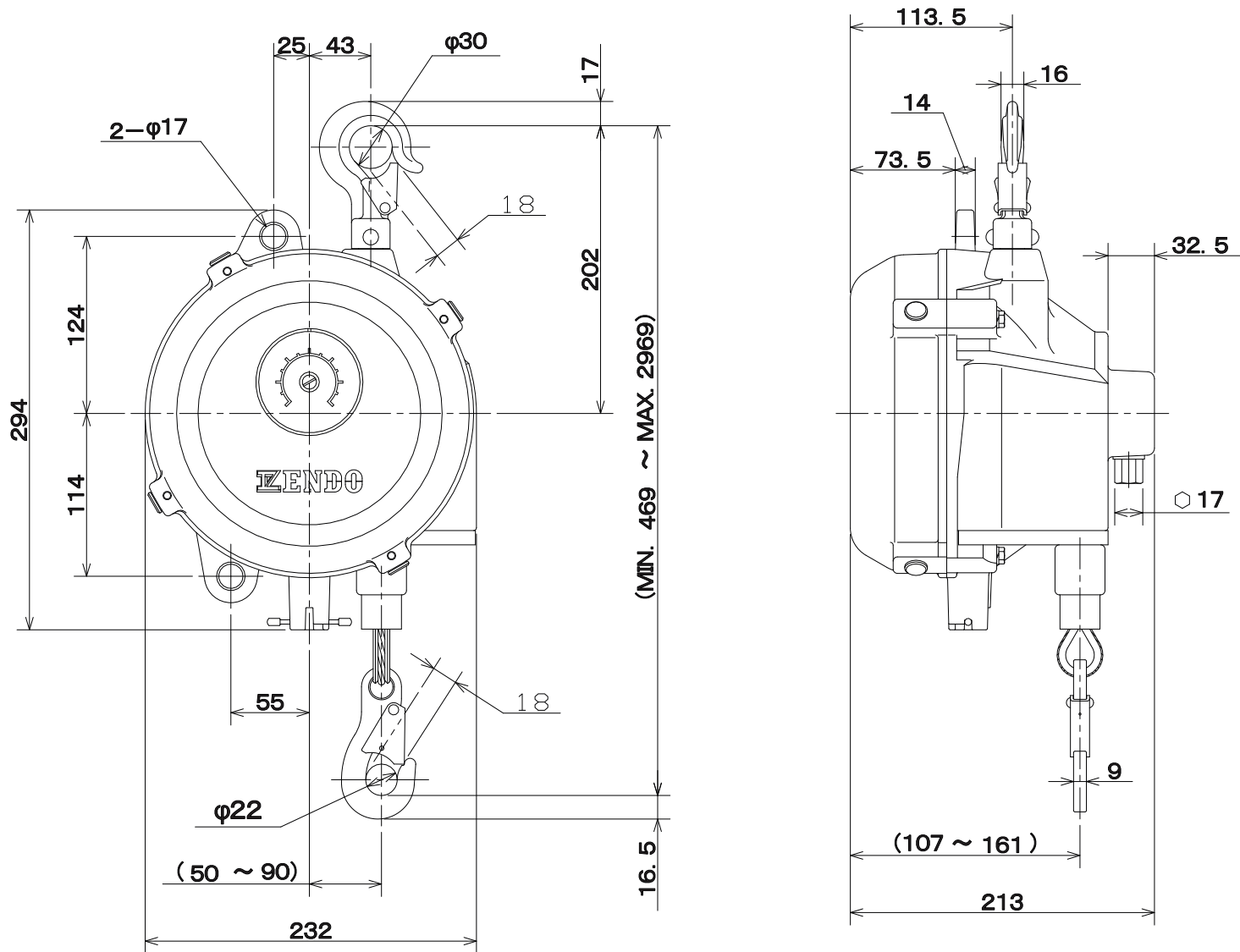
SPRING BALANCER ELF-15
